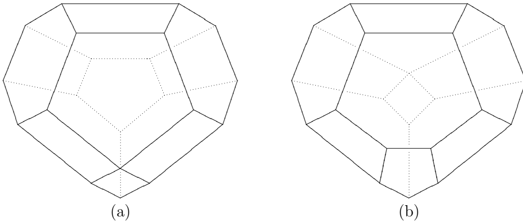
Figure 1: The main character: Two views of the 3-d multiplihedron \mathcal{J}(4) .
