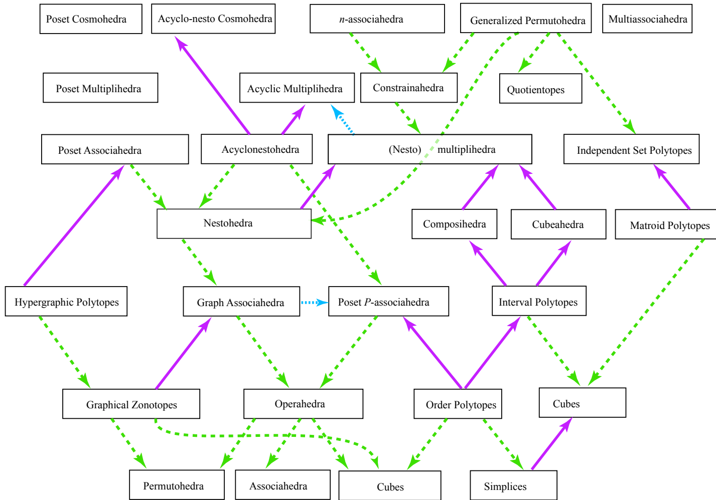
Figure 1: Some families of combinatorial polytopes. Green arrows point in the direction of subset containment: lower contained in upper. Purple arrows show lifting, or collapse (in reverse). Dashed blue arrows indicate taking a cross section. No arrows at all means the family of polytopes is conjectural.
